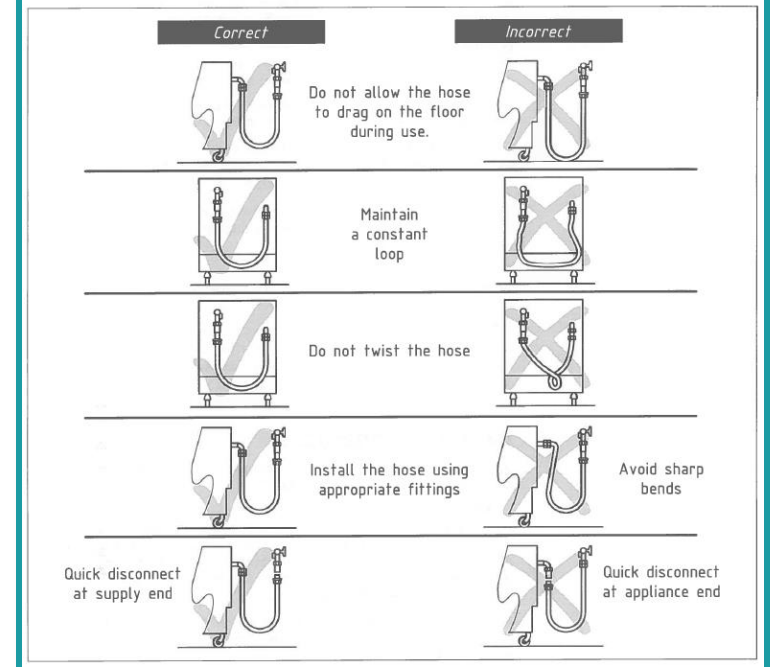
Figure 1 Guidance on installation of flexible connection
